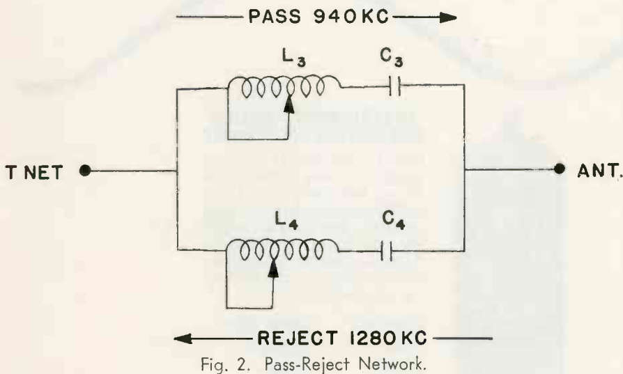
Fig. 2. Pass-Reject Network.
