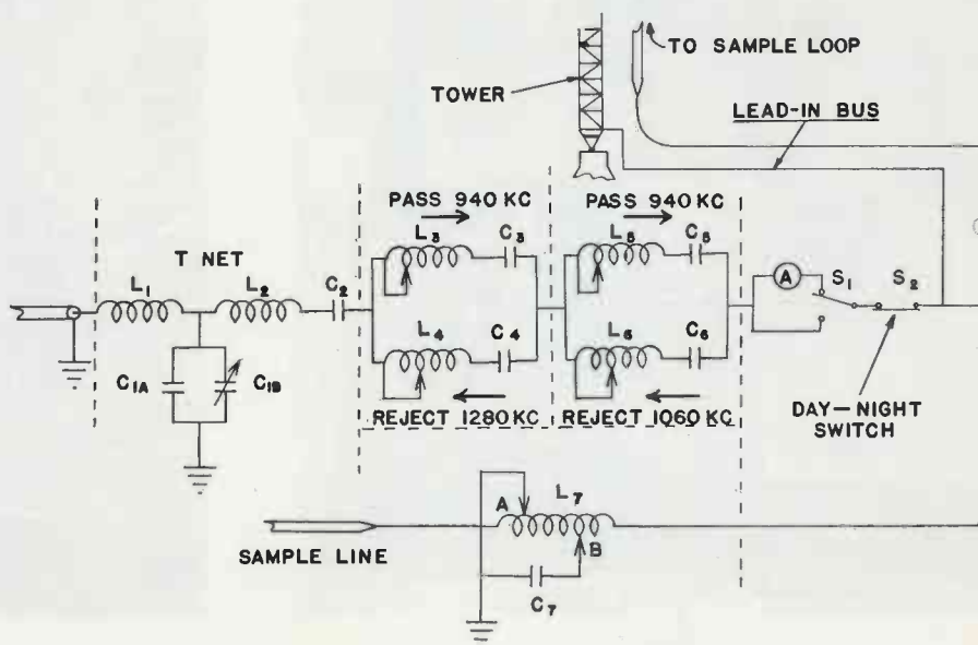
Fig. 4b. Antenna Tuning Unit Schematic.
