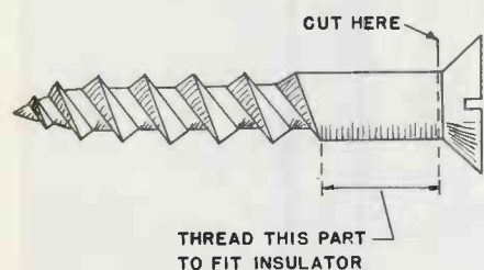
Fig. 4a. Special Screw.
