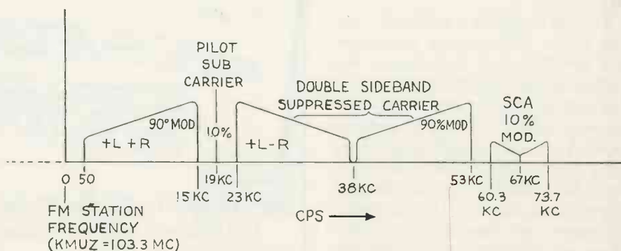
Fig. 1. Distribution of channels and frequencies in standard stereo carrier.
