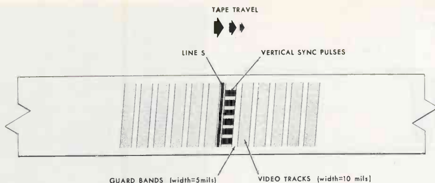
Fig. 3. Detail of "splicing" point.
